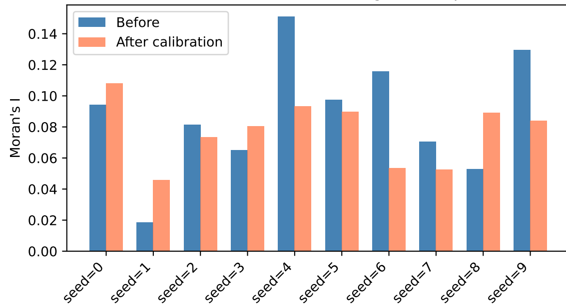
Moran's I: before vs after — ('german', 'platt')
